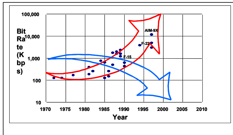
Figure 2: TM demand increasing while supply decreases
